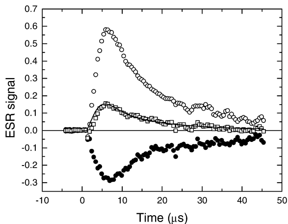
Figure 3. Pulse radiolysis of 5 mM aqueous solutions of \alpha -(methylthio)acetamide, N_2O -saturated, at pH 7 (phosphate buffer). TRESR kinetic traces of two matching lines: high-field line ( \circ ) at \Delta H_0 = 12.85 G and low-field line ( \bullet ) at \Delta H_0 = -21.66 G, and the average of the two traces ( \square ). The solid curve is the kinetic simulation from the modified Bloch equations, with [primary radicals] = 40 \mu M , T_1 = T_2 = 2.2 \mu s , 2k_2 = 2.2 \times 10^9 M^{-1} s^{-1} , k_1 = 5 \times 10^4 s^{-1} , W = 23.5 mG, H_1 = 16 mG, and scale factor = 0.0125 \times 48 lines = 0.6, based on a full yield from \bullet OH radicals. The reference scale factor = 5.0 for SO_3^{\bullet -} .
